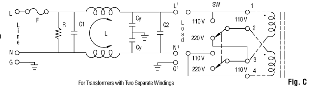
For Transformers with Two Separate Windings
